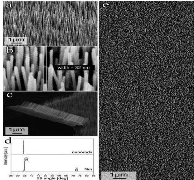
Figure 3: SEM images of the obtained arrays of vertically aligned ZnO nanorods: (a) tilted the view; (b) higher magnification image with the typical size of a nanorod; (c) cross-section view of a fractured zone, where the ZnO film-rod structure is clearly visible. (d) XRD spectra of a seeding ZnO film before and after the growth of ZnO nanorods; preferential orientation along the c-axis of the wurtzite hexagonal structure is clearly visible in both samples. (e) SEM top view image that shows vertical alignment and planar distribution [17]
