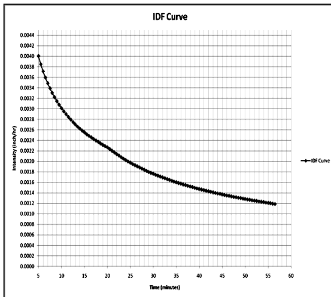
Figure 1: Intensity-Duration-Frequency Curve
